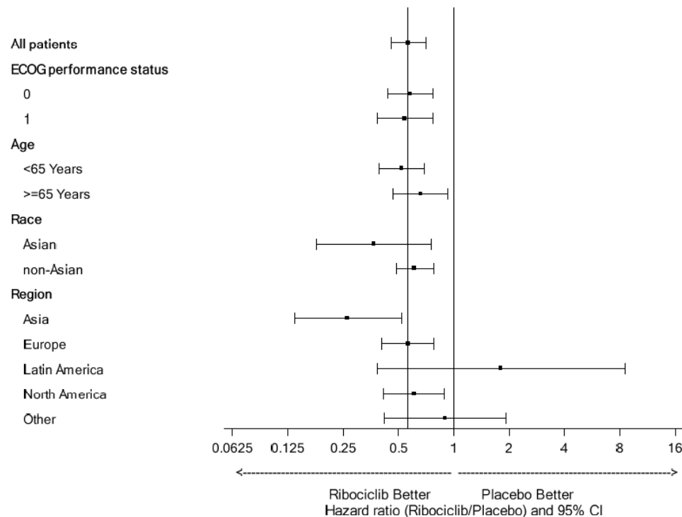
Figure 2 MONALEESA-2 (A2301) Forest plot of PFS based on Investigator assesment (FAS) (02 January 2017 cut-off)
